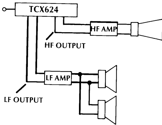
Bi-Amplified System
