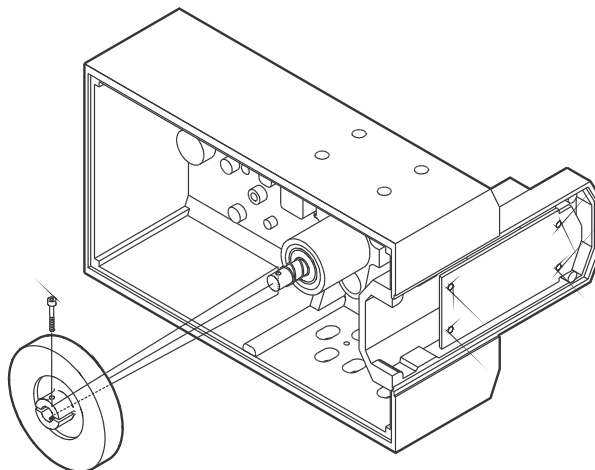
Figure 2.2 Flywheel Mounting
